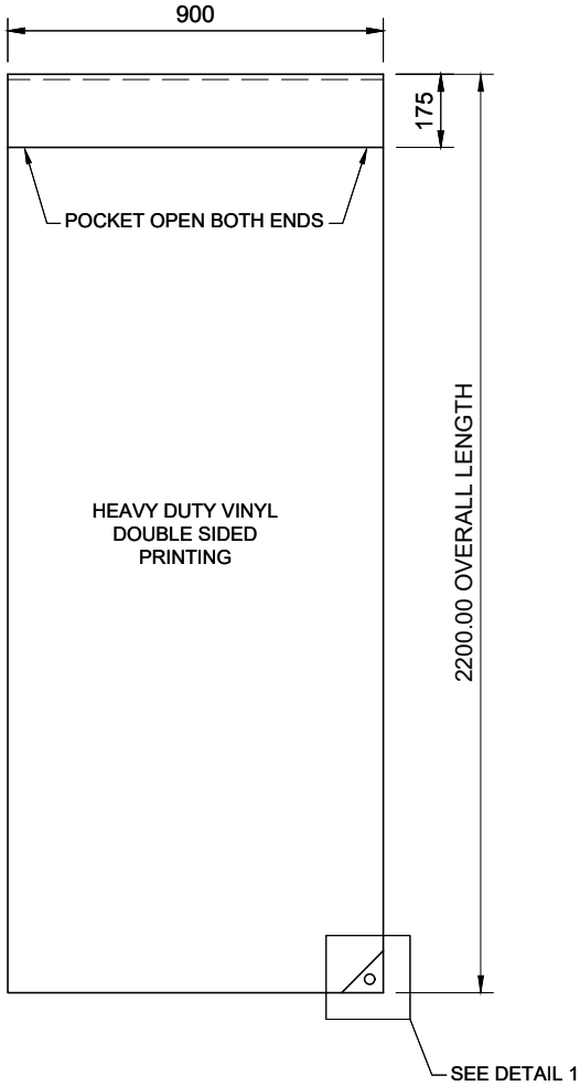
FRONT VIEW
