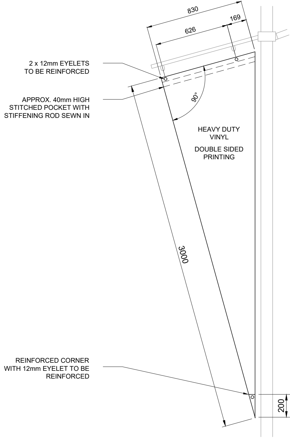
FRONT VIEW
