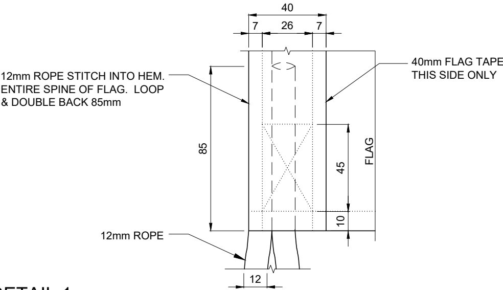
DETAIL 1
