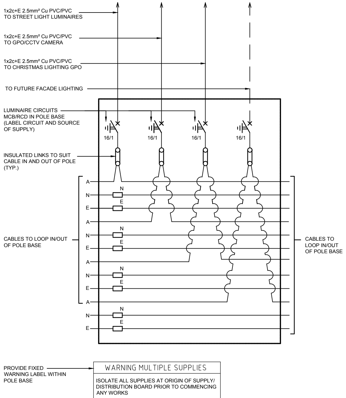
TYPICAL WIRING SCHEMATIC NOT TO SCALE
