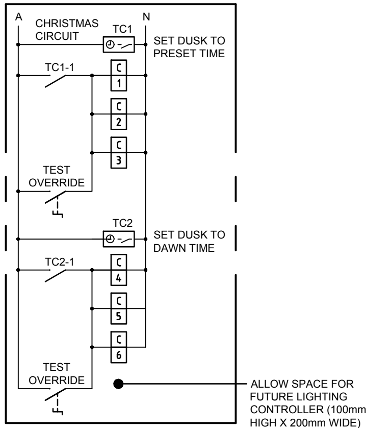
LIGHTING CONTROL NOT TO SCALE
