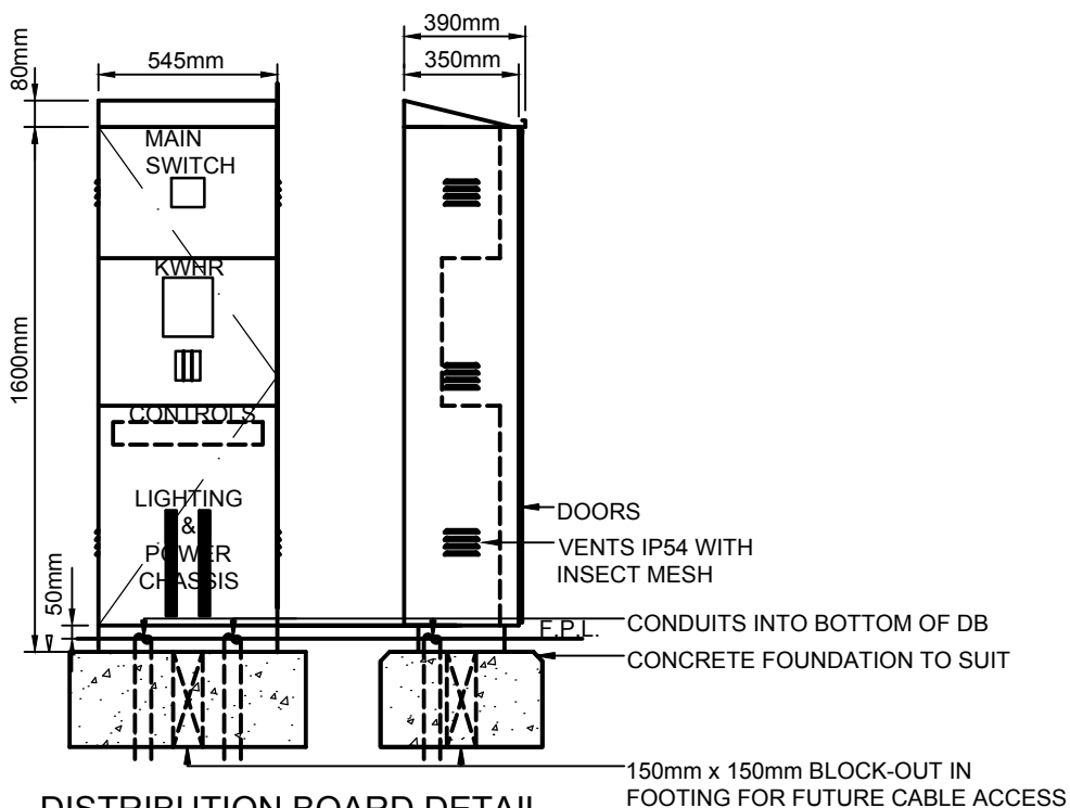
DISTRIBUTION BOARD DETAIL NOT TO SCALE
