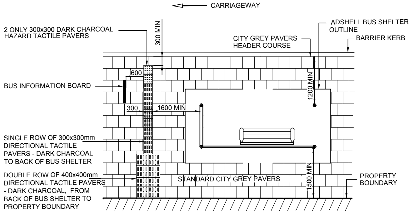
TYPICAL BUS STOP AND TACTILE PAVERS WITH BUS SHELTER
