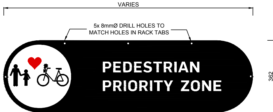
TYPICAL SIGNAGE PANEL GRAPHIC TYPE / TEXT SCALE 1:10
