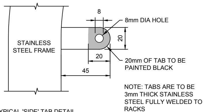
TYPICAL 'SIDE' TAB DETAIL
