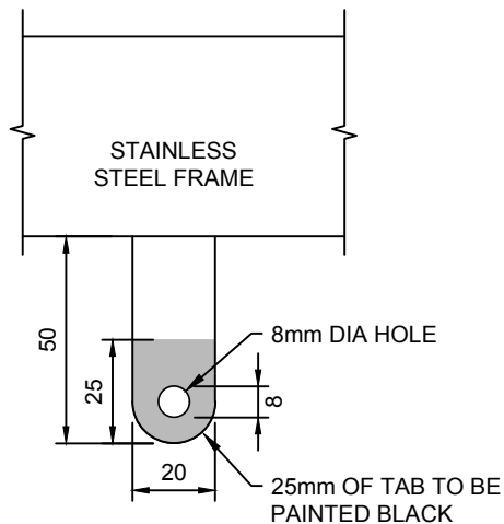
TYPICAL 'TOP' TAB DETAIL
