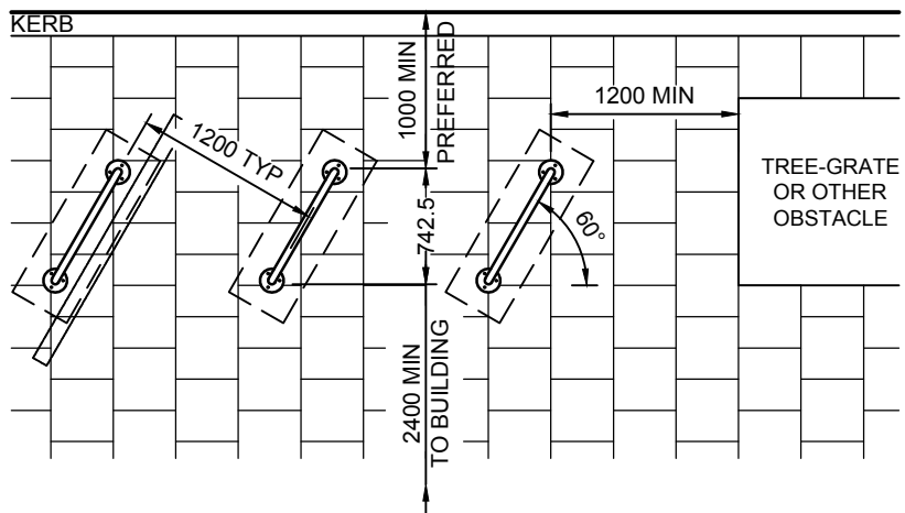
BIKE RACKS 60° ANGLE TO KERB
