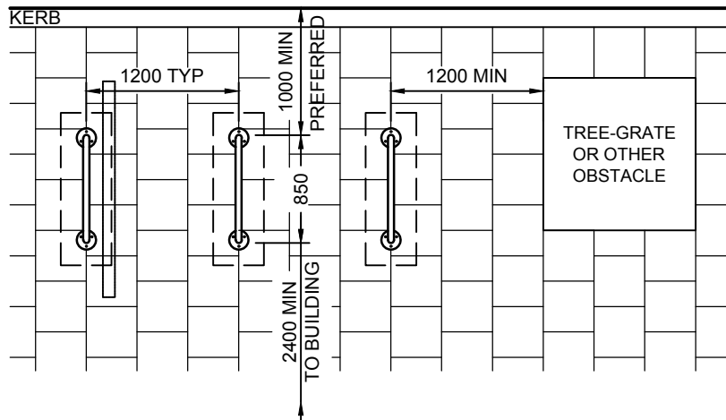
BIKE RACKS PERPENDICULAR TO KERB
