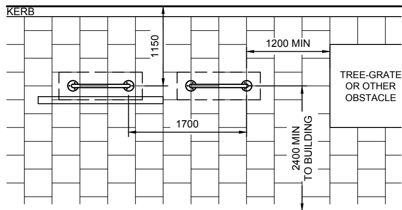
BIKE RACKS PARALLEL TO KERB
