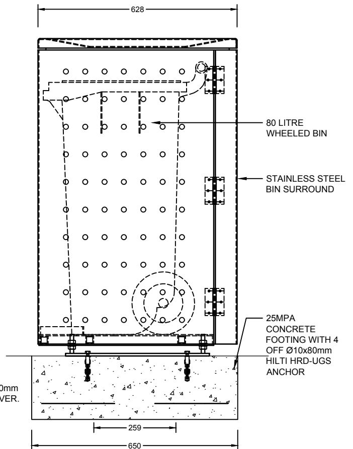
SIDE ELEVATION
